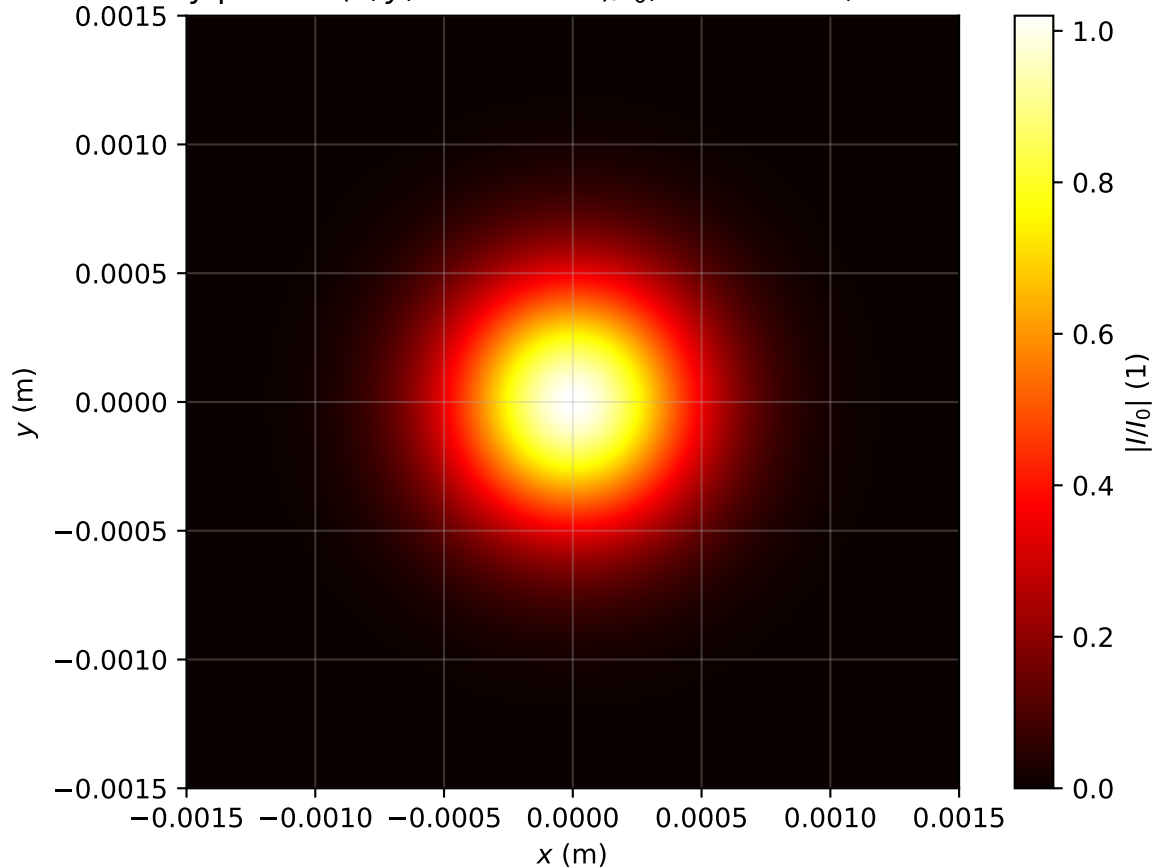
Intensity profile I(x, y, z = 0.478m)/I_0 , P_{in}=0.4P_{cr} , artificial time
